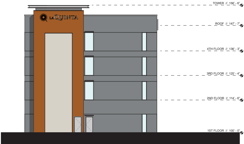
RIGHT ELEVATION: 4 STORIES
